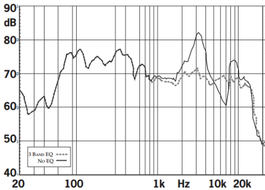
Frequency Response - Typical Glass SolidDrive Response
